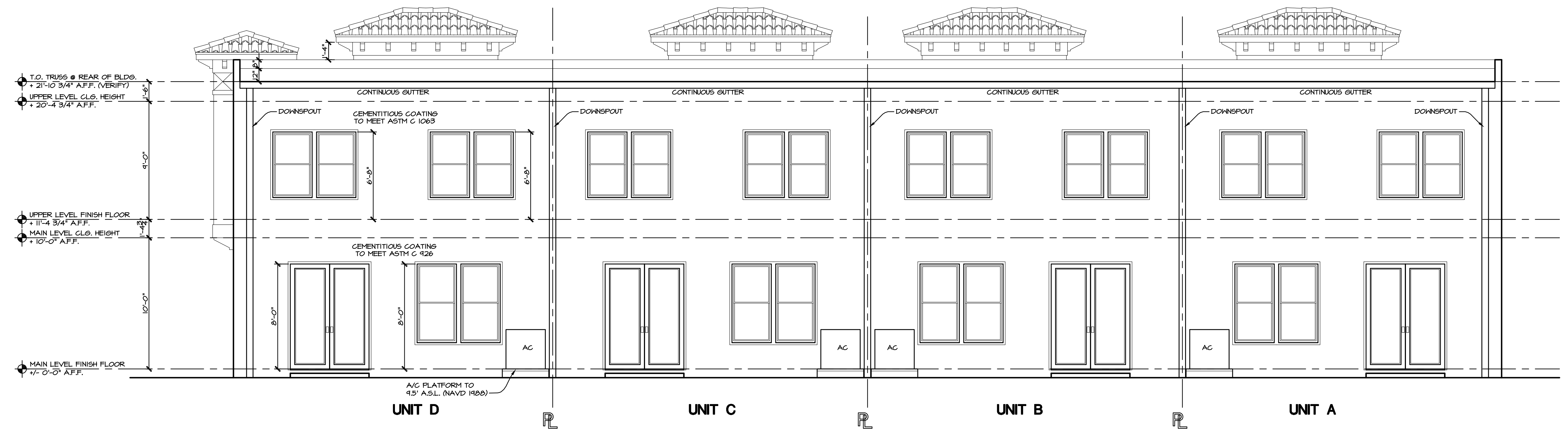
REAR (EAST) ELEVATION SCALE 1/4" = 1'-0"
