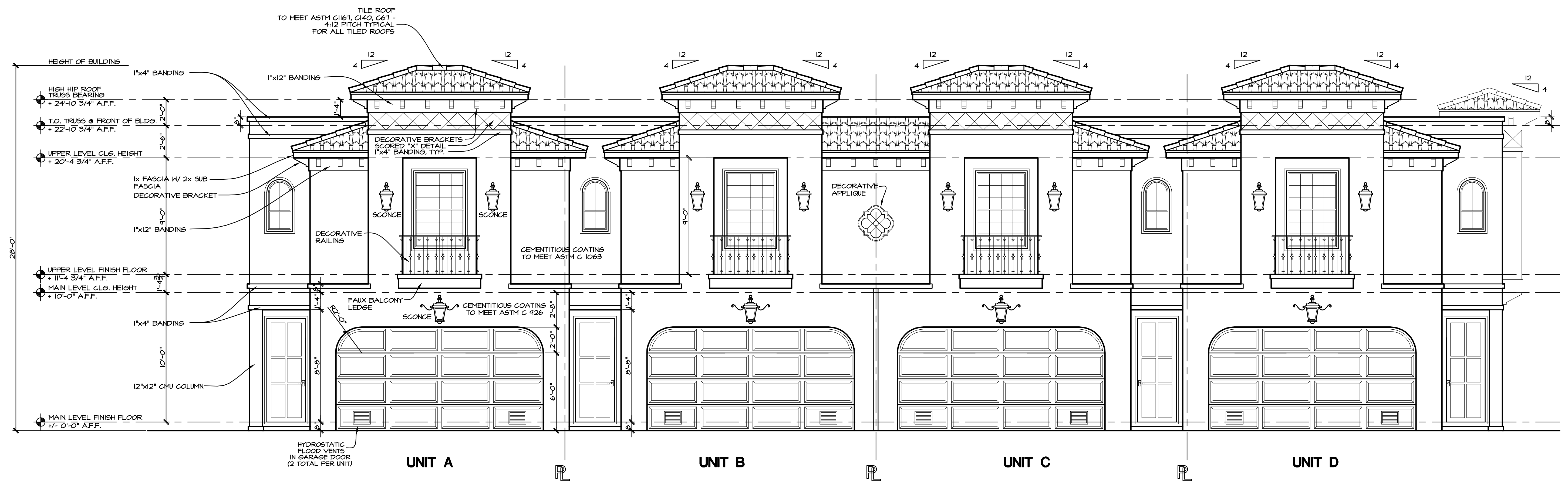
FRONT (WEST) ELEVATION SCALE 1/4" = 1'-0"
